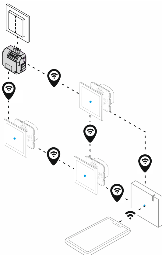
Fig. 9: Home automation expansion stage (home control)
