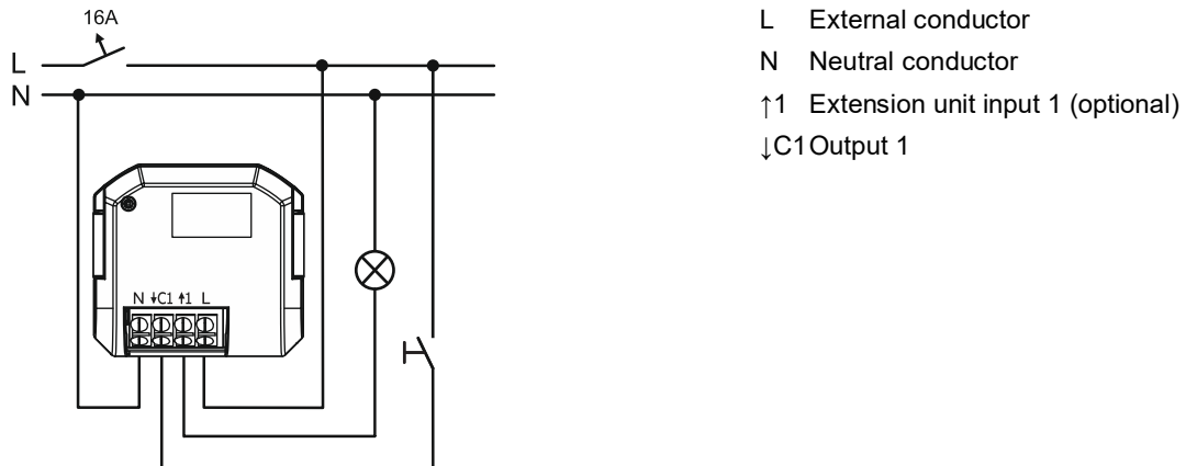
Fig. 5: Electrical connection 62811 U-WL-500
